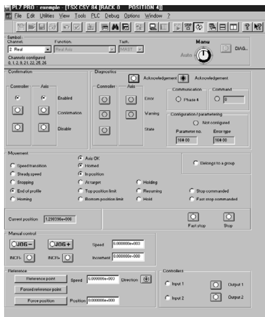
Debugging in PL7 Pro software
