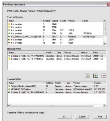
Fieldbus lookup screen
