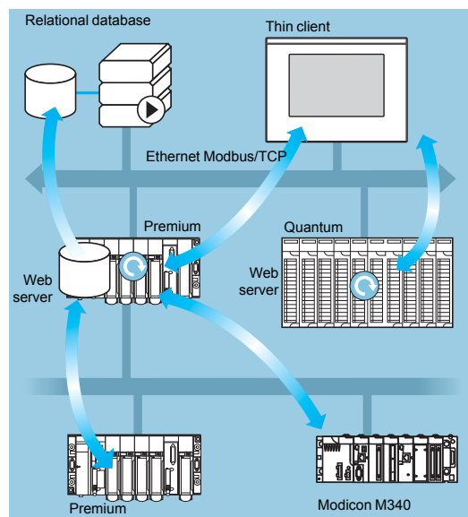
Flexible distributed HMI solution
