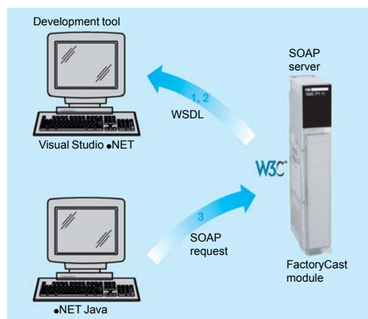
ModbusXMLDa server interface
