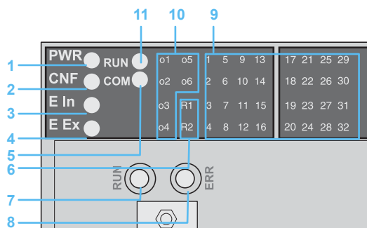
Illuminated display
