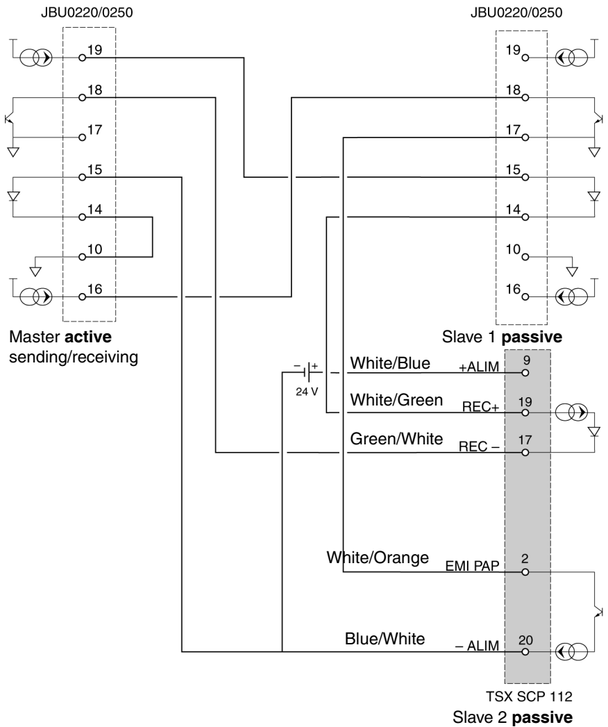
Example 2: active send/receive JBU0220/0250 multidrop
